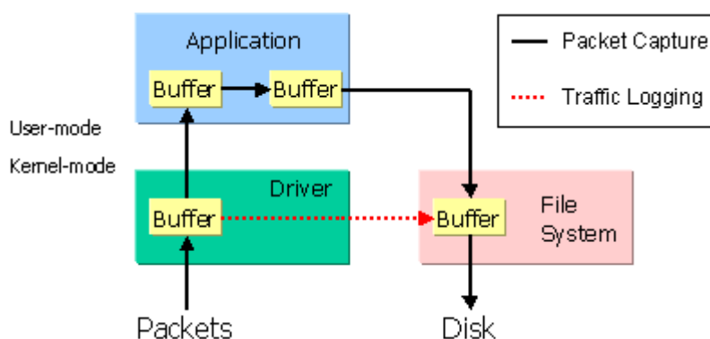
Figure 32: Packet Capture vs. Kernel-Level Dump
