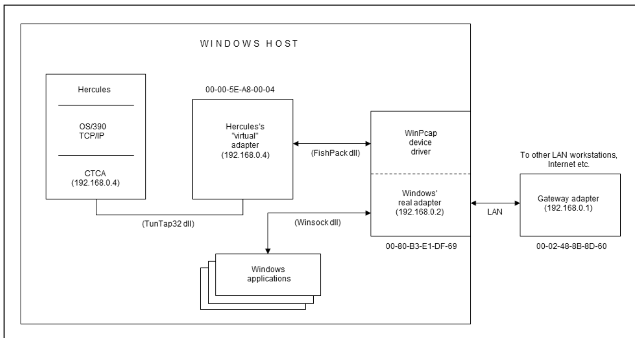
Figure 33: CTCI-WIN Implementation
