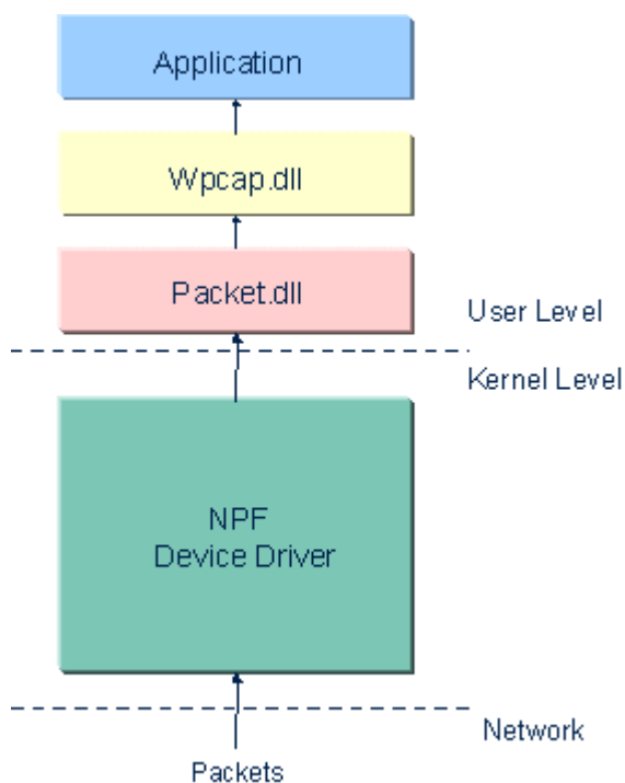
Figure 29: WinPcap Architecture
