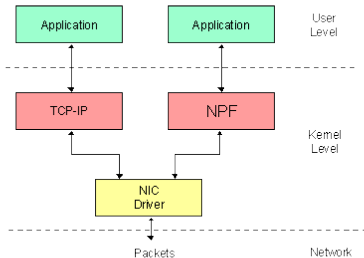
Figure 30: NPF inside NDIS
