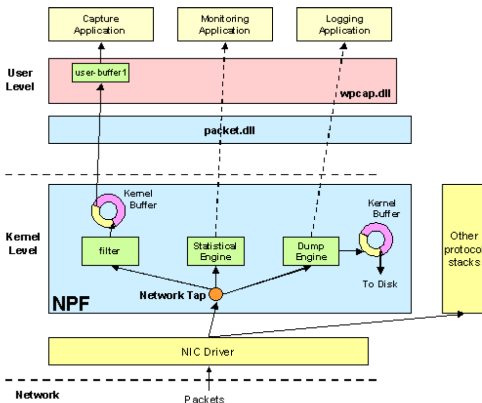
Figure 31: NPF Device Driver
